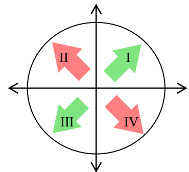
tangent
